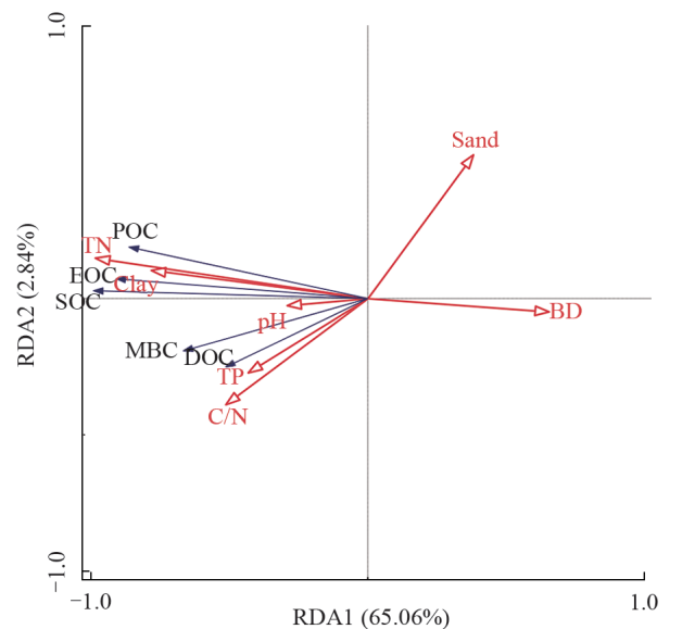
图 6 土壤理化性质对土壤有机碳组分影响的冗余分析 Fig. 6 Redundancy analysis of effects of soil physicochemical properties on soil organic carbon fractions
