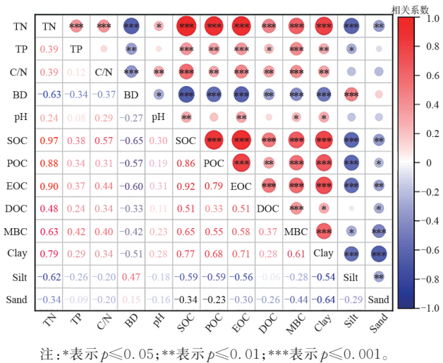
图 5 土壤有机碳组分与土壤理化性质的相关关系 Fig. 5 Correlation between soil organic carbon fractions and soil physicochemical properties
