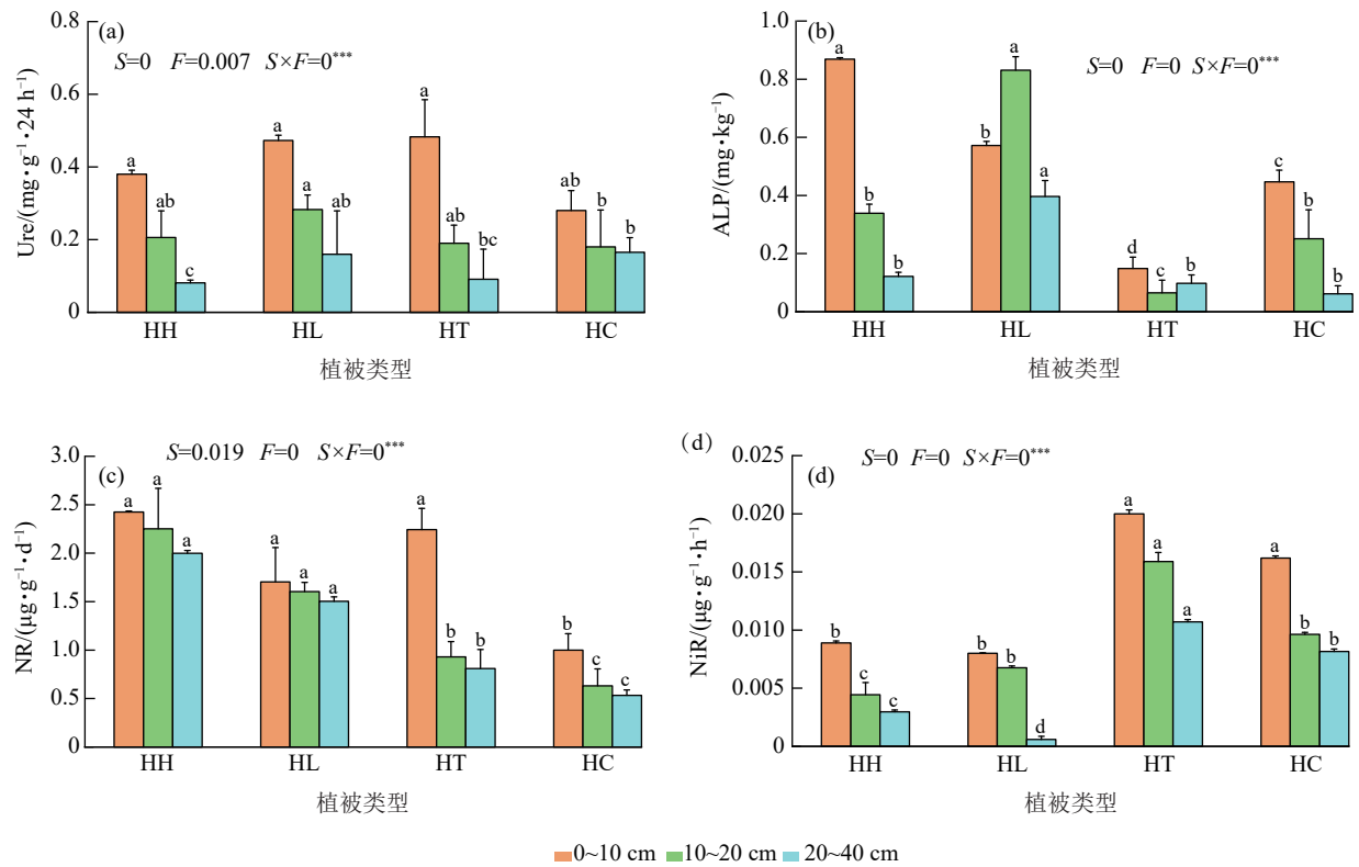
Fig. 1 Basic physical and chemical properties of soils at four vegetation types
