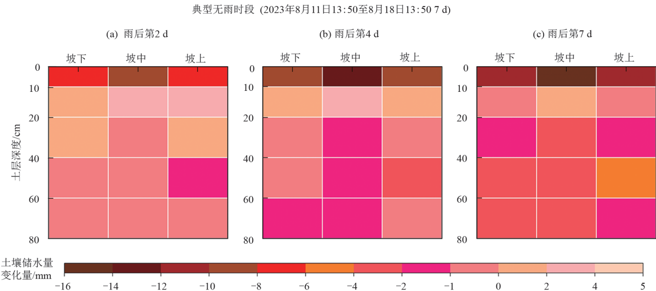
图 5 典型无雨时段下不同坡位各土层土壤储水量变化过程 Fig. 5 Changes in soil water storage in different soil layers at different slope positions during a typical dry period
