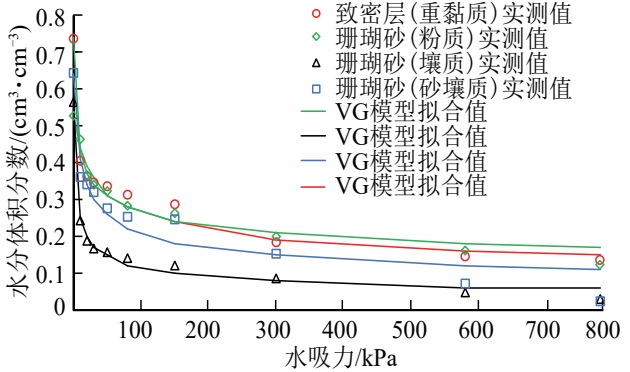
图 2 4 种典型质地珊瑚砂的水分特征曲线 Fig.2 Moisture characteristic curves of four typical coral sand textures
