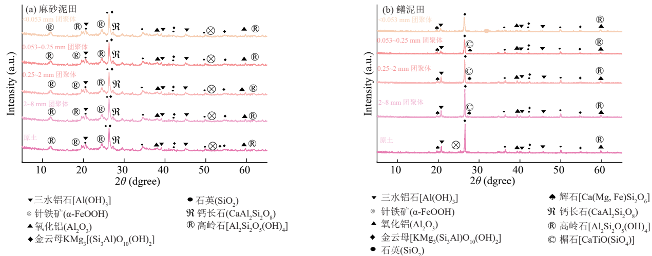
图 2 麻砂泥田与鳊泥田各粒级团聚体矿物组成 Fig. 2 Mineral compositions of aggregates with different particle sizes in granitic sandy soil and eel clayey soil
