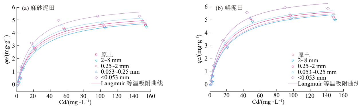
图 8 去除游离氧化铁土壤团聚体对外源 Cd 的等温吸附模型 Fig. 8 Isothermal adsorption models for exogenous Cd onto soil aggregates after free iron oxide removal
