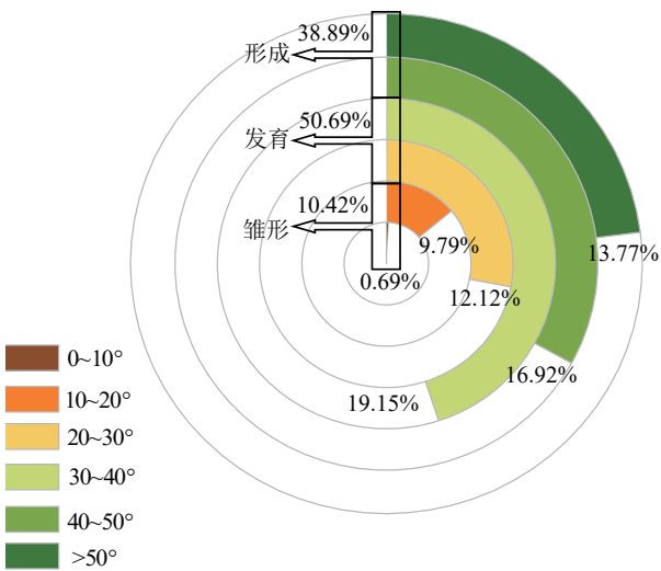
图 4 龕穴角度占比与发育状态 Fig. 4 Proportion of niche angles and developmental status
