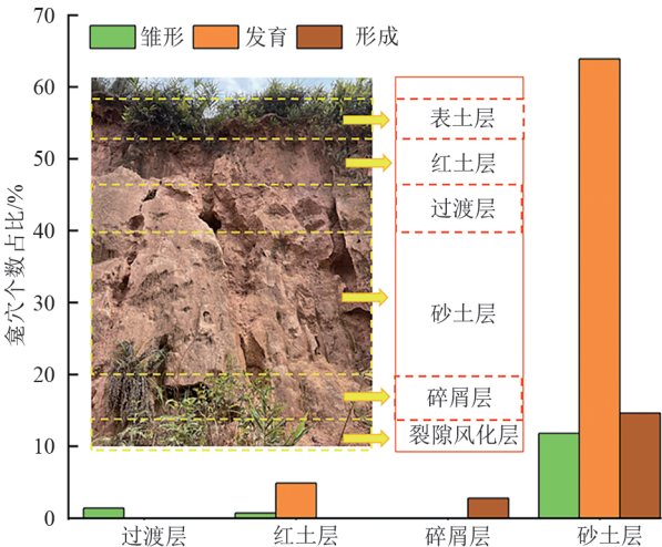
注: n=144 。 图 5 不同土层发育的龕穴个数占比及其发育状态 Fig. 5 Proportions of niches developed in different soil layers and in their developmental status
