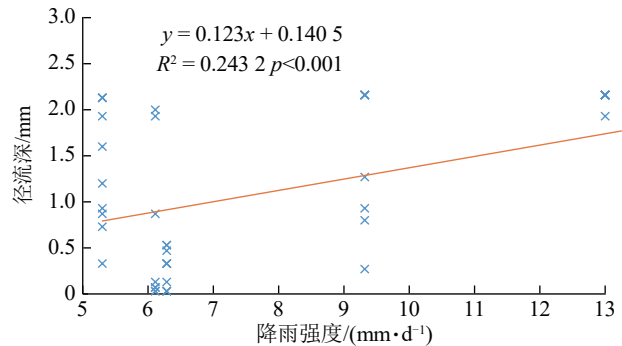
图 5 降雨强度与径流深的函数关系 Fig. 5 Functional relationship between rainfall intensity and runoff depth
