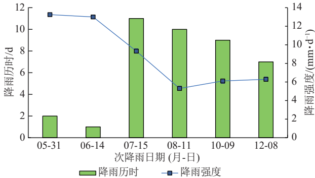
图 4 次降雨历时与降雨强度 Fig. 4 Duration and intensity of individual rainfall events
