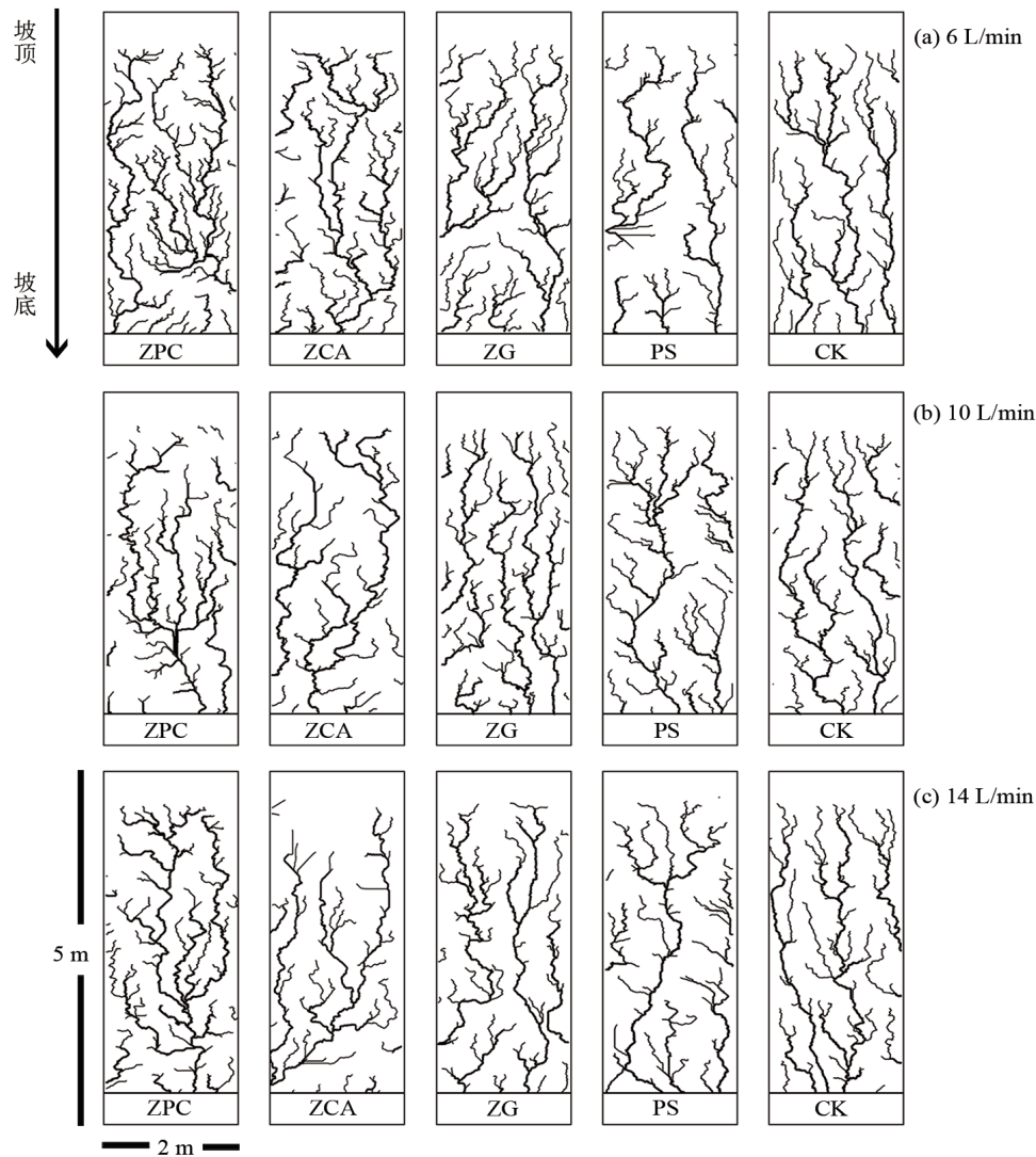
图 6 汇流网络演变特征 Fig. 6 Evolutionary characteristics of the runoff network
