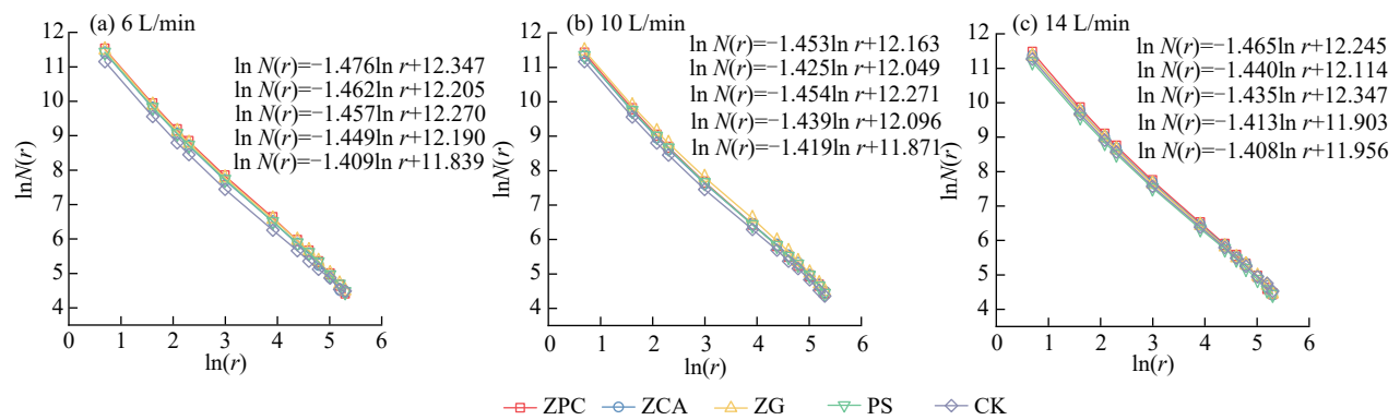
图 6 汇流网络演变特征 Fig. 6 Evolutionary characteristics of the runoff network
