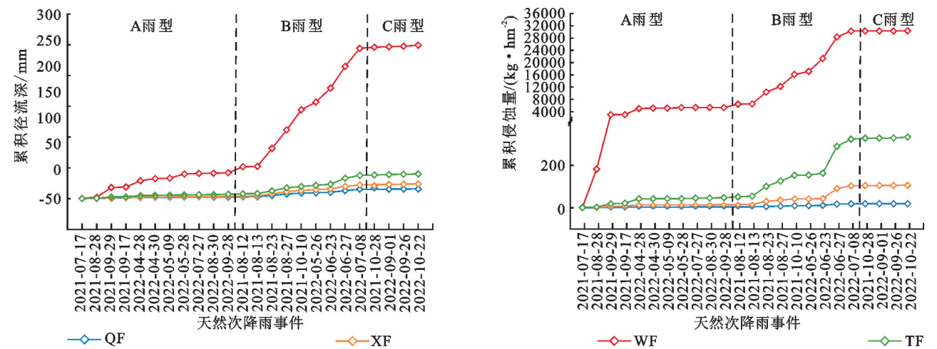
图 3 不同林草覆被格局的累积径流深与累积土壤侵蚀量 Fig. 3 Cumulative runoff depth and soil erosion for the different vegetation cover patterns
