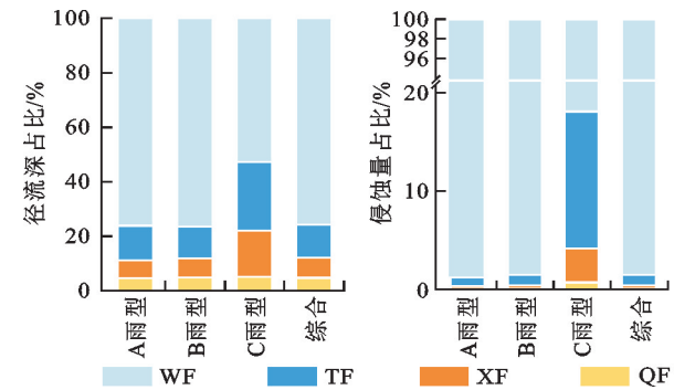
图 4 不同林草覆被格局径流深和侵蚀量占比 Fig. 4 Percentage of runoff depth and erosion amount for the different vegetation cover patterns
